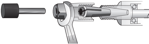
Figure 16. Collet chuck.
