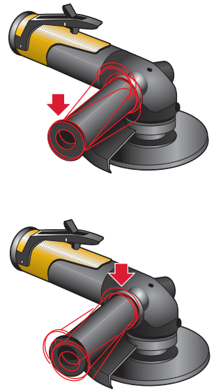
Figure 50. Vibration-damped handle
